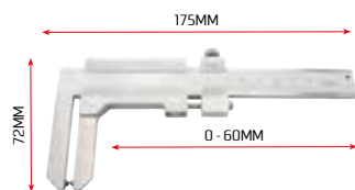
SGO #47024 Stainless steel vernier caliper for disc brakes
