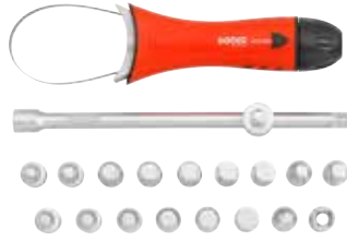
#302001 Oil drain set 1/2", 20-pcs Included metal band filter wrench ø60-120
