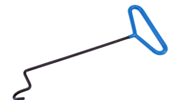
#47815 Doughnut stretcher For removing the retaining rubbers on exhaust systems.
