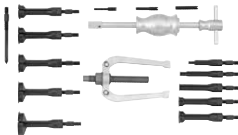
SGO #818021 Blind hole bearing puller set, 16-pcs
