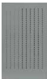
#47292 845mm wall cabinet Dimensions: W 674 x D 300 x H 400mm
