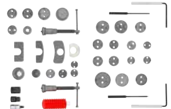
#809007 Brake caliper set, 40-pcs
